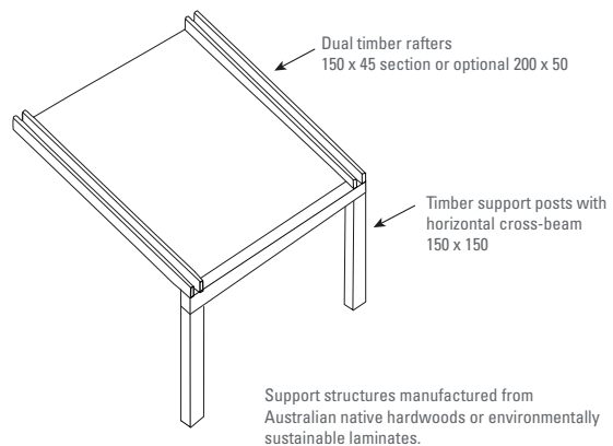
Traditional Fleetwood support structure
