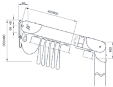
Typical fixing detail
