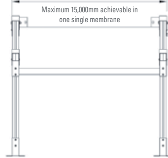
Maximum width 5,000mm centre/centre of runner
